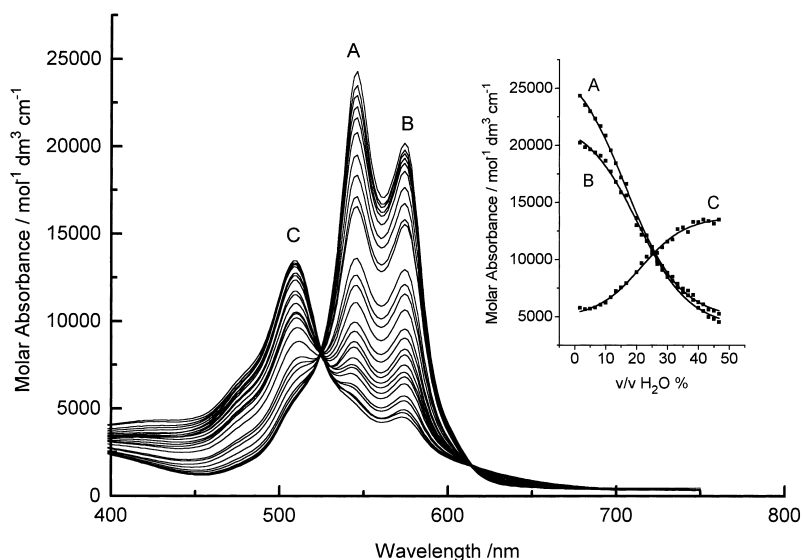
Fig. 6. UV-vis absorption spectra of [\text{Mn}_2 \cdot \mathbf{2}](\text{OAc})_2 ( 5.75 \times 10^{-5} M) in a \text{CH}_3\text{OH}:\text{H}_2\text{O} mixture ranging from 0 to 50% \text{H}_2\text{O} v/v illustrating the decrease in the absorptions at 546 and 574 nm and increase of the absorption at 510 nm with increased percentage of \text{H}_2\text{O} at 21^\circ\text{C} . Inset shows the molar absorbances found at the peaks 510 (C), 546 (A), and 574 nm (B) vs. % \text{H}_2\text{O} .
