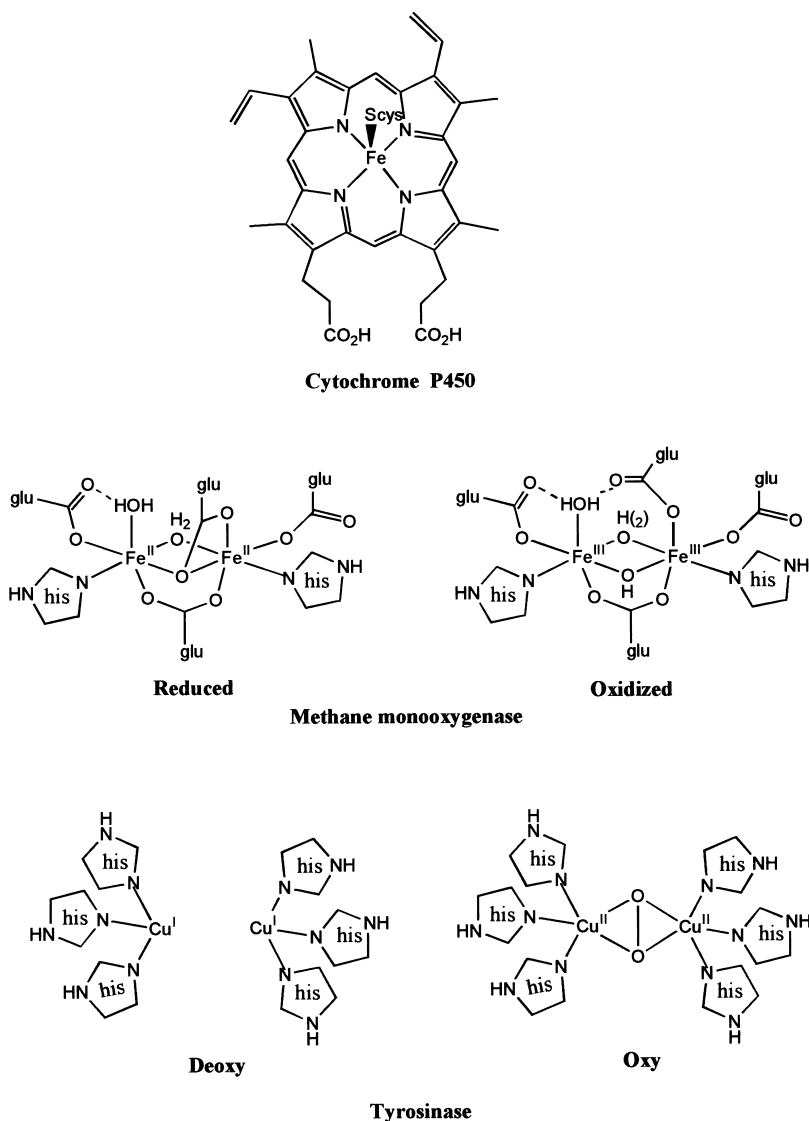
Fig. 1. Active sites for cytochrome P450, methane monooxygenase, and tryosinase.
